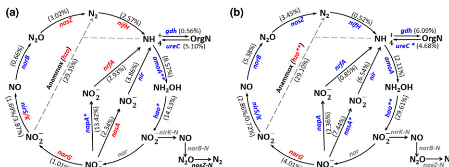
FIGURE 4 The fold change of nitrogen cycle genes by (a) soil erosion and (b) soil deposition. The percentage of each gene indicates the extent of fold change, with red and blue colours representing increase and decrease, respectively. The percentage was calculated by relative abundance of each gene at the eroded or deposited site divided by the control. Asterisk indicates significant differences. * p < .05 ; ** p < .01 [Colour figure can be viewed at wileyonlinelibrary.com ]
