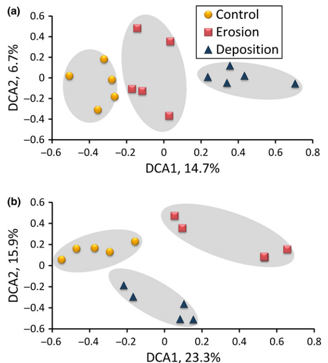
FIGURE 1 The detrended correspondence analysis (DCA) of (a) taxonomic structure and (b) functional structure. The values of axes 1 and 2 are percentages of community variation attributed to the corresponding axis. [Colour figure can be viewed at wileyonlinelibrary.com ]
