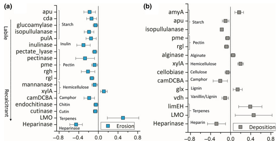
FIGURE 3 The response ratio analysis to detect changes of bacterial carbon degradation genes by (a) soil erosion and (b) soil deposition. Only significant changes at the confidence level of 0.90 are shown [Colour figure can be viewed at wileyonlinelibrary.com ]
