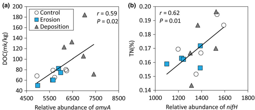
FIGURE 5 Pearson correlations between (a) relative abundance of amyA and DOC; and (b) relative abundance of nifH and TN. DOC, dissolved organic carbon; TN, total nitrogen [Colour figure can be viewed at wileyonlinelibrary.com ]
