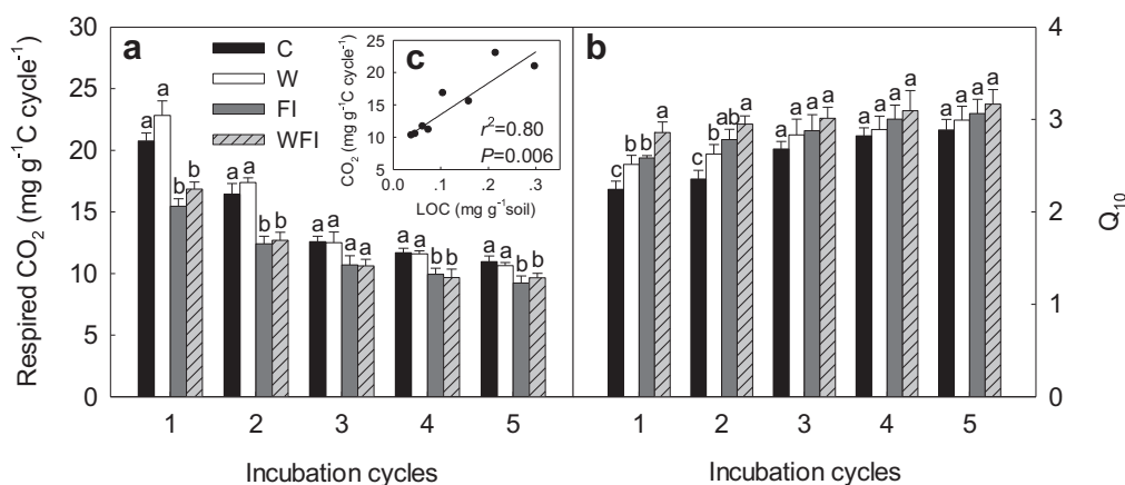
Fig. 2. Variation in SOC decomposition (expressed as respired \text{CO}_2 , a) and Q_{10} values (b) over lab incubation cycles under four treatments. The insert panel (c) shows a correlation between LOC content (before and after lab incubation) and respired \text{CO}_2 in the 1st and 5th incubation cycles ( n = 8 ). C: control (ambient) temperature and normal litter input; W: field warming and normal litter input; FI: control temperature and field incubation (9 years' litter exclusion); WFI: field warming and field incubation.
