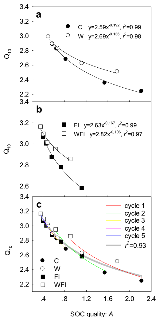
Fig. 3. The negative relationships between SOC quality (A) and the Q_{10} of SOC decomposition under different treatments over all incubation cycles (a, b) and under different incubation cycles over all treatments (c). Different color lines in panel (c) represent curves fit within each lab incubation cycles ( n = 4 ). The gray line shows an overall relationship between SOC quality and the Q_{10} values across all treatments and incubation cycles ( n = 20 ). Data were fit using the two-parameter power equation: Q_{10} = a \times A^k . See Fig. 2 for acronyms (C, W, FI, and WFI).
