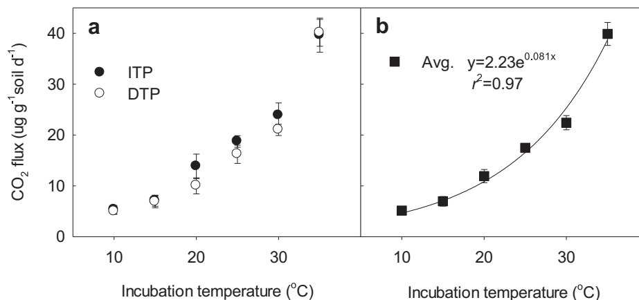
Fig. 1. An example of Q_{10} value calculation of SOC decomposition by curve fitting. No statistically significant differences were found at any specific incubation temperature between increasing temperature period (ITP) and decreasing temperature period (DTP) (a), we thus averaged the respiration values at each temperature when fitting the curve to get Q_{10} values (b, Fang et al., 2005). Values are mean \pm SE ( n = 6 ) from the first incubation cycle under control treatment. Q_{10} values based on the fitted curves with respiration rates from ITP, DTP, and averaged values were not significantly different from each other (all P > 0.05 ).
