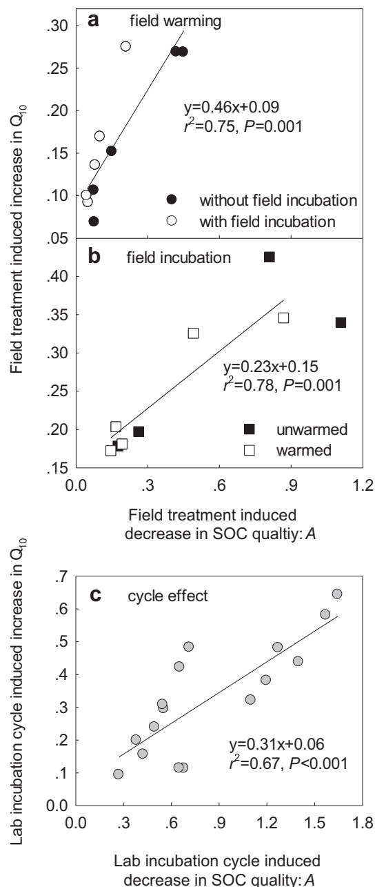
Fig. 4. Relationships of the changes in SOC quality (A) and Q_{10} values under field warming (a, n = 10 ), field incubation (b, n = 10 ), and different laboratory incubation cycles across all treatments (c, n = 16 ). Incubation-cycle effects in panel c represent the differences of the 1st incubation cycle with the following four (2nd–5th) cycles.
